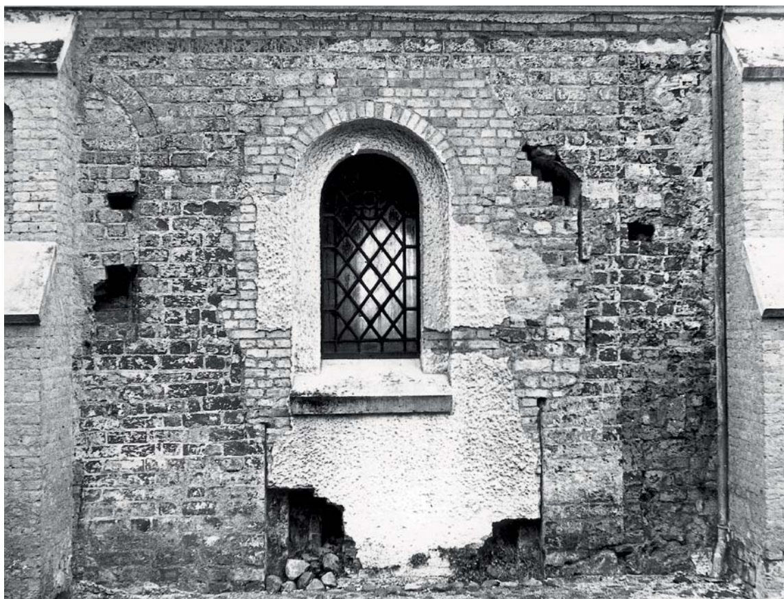
Fig. 17. Nordsiden af skibets østfag under renovering. Kirkens oprindelige norddør ses under vinduet fra 1878. Øst for vinduet er det oprindelige vindue delvist dækket af støttepille fra 1878, mens resterne af et fladbuet vindue fra 1823 er lokaliseret vest for vinduet. Yderligere vest herfor ses i murværket spor af den nedbrudte, oprindelige støttepille. Foto i NM, 1961. – The north side of the east bay of the nave during renovation. The original north door of the church can be seen beneath the window from 1878. East of the window the original window is partly covered by the buttress from 1878, while the remains of a low-arched window from 1823 have been localized west of the window. Farther west from this, in the masonry, one can see traces of the demolished original buttress.
